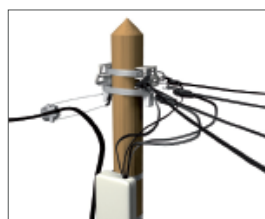
Branchement multiple
